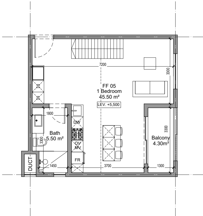
FIRST FLOOR [APARTMENT 5]
